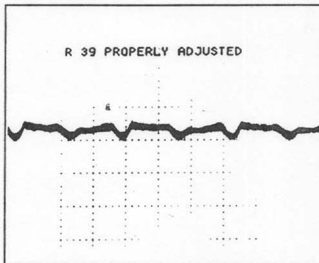
Figure 7 Results with Properly Adjusted LF Cancel
