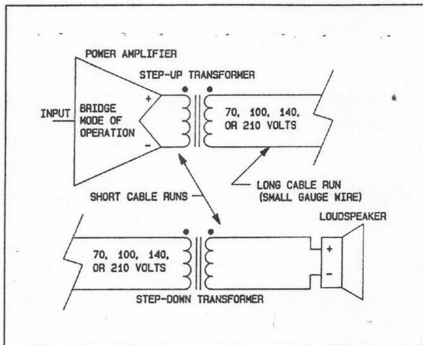
Figure 5 High-voltage Distribution System
